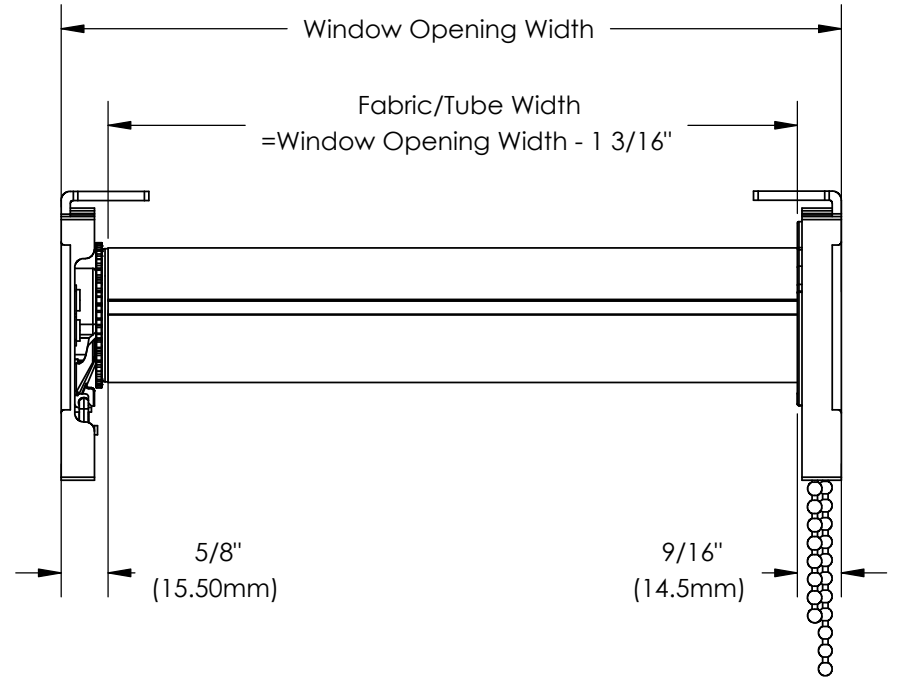
RA-CM system( without end cap) light gap & Fabric/Tube deduction
