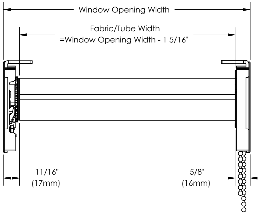
RA-CM system( with end cap) light gap & Fabric/Tube deduction
